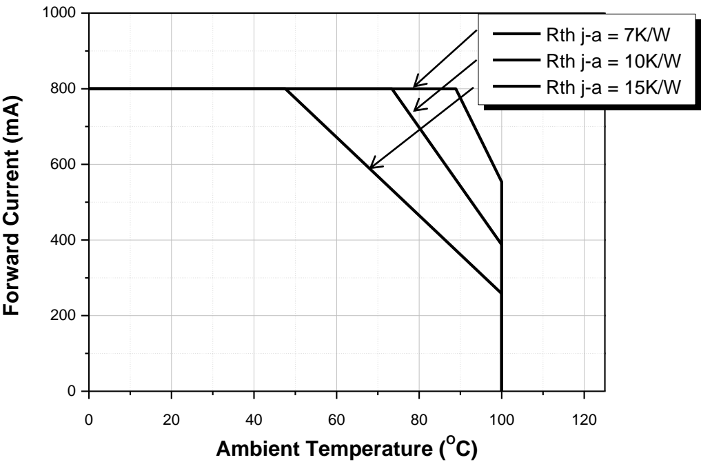
Fig 9. Maximum Forward Current vs. Ambient Temperature, T_j(max.)=125^{\circ}C , I_F=800mA
